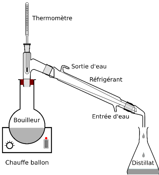
Figure 3 : Distillation simple
